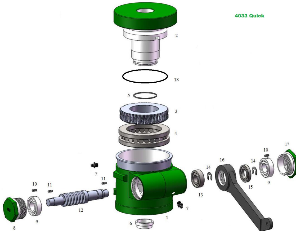
4033 Rod Rotator Diagram
