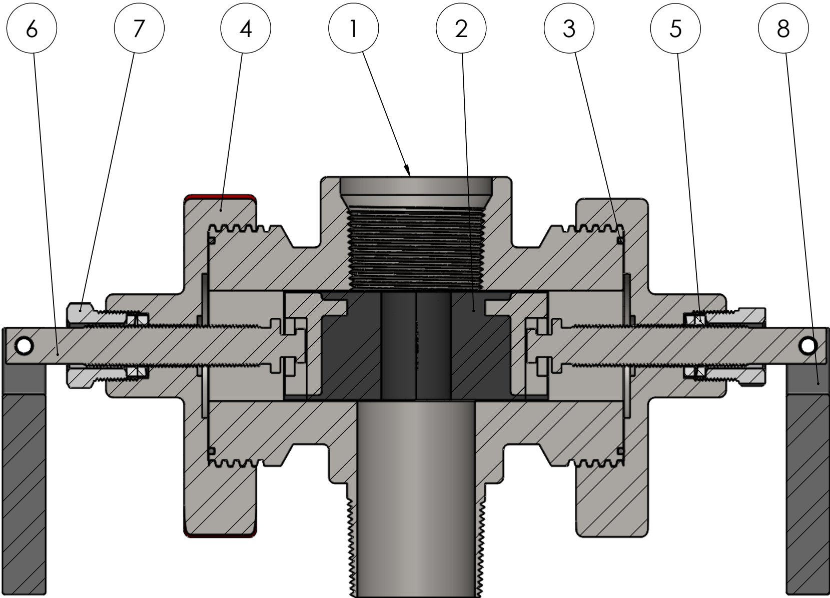
SECTION AA-AA SCALE 1 : 2
