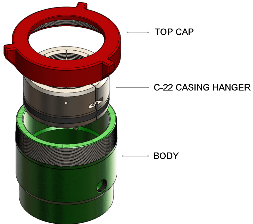
MODEL "92" CASING HEAD C-22 PROFILE
