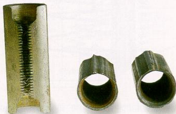
An example of coupling wear as a result of not running rod rotators
