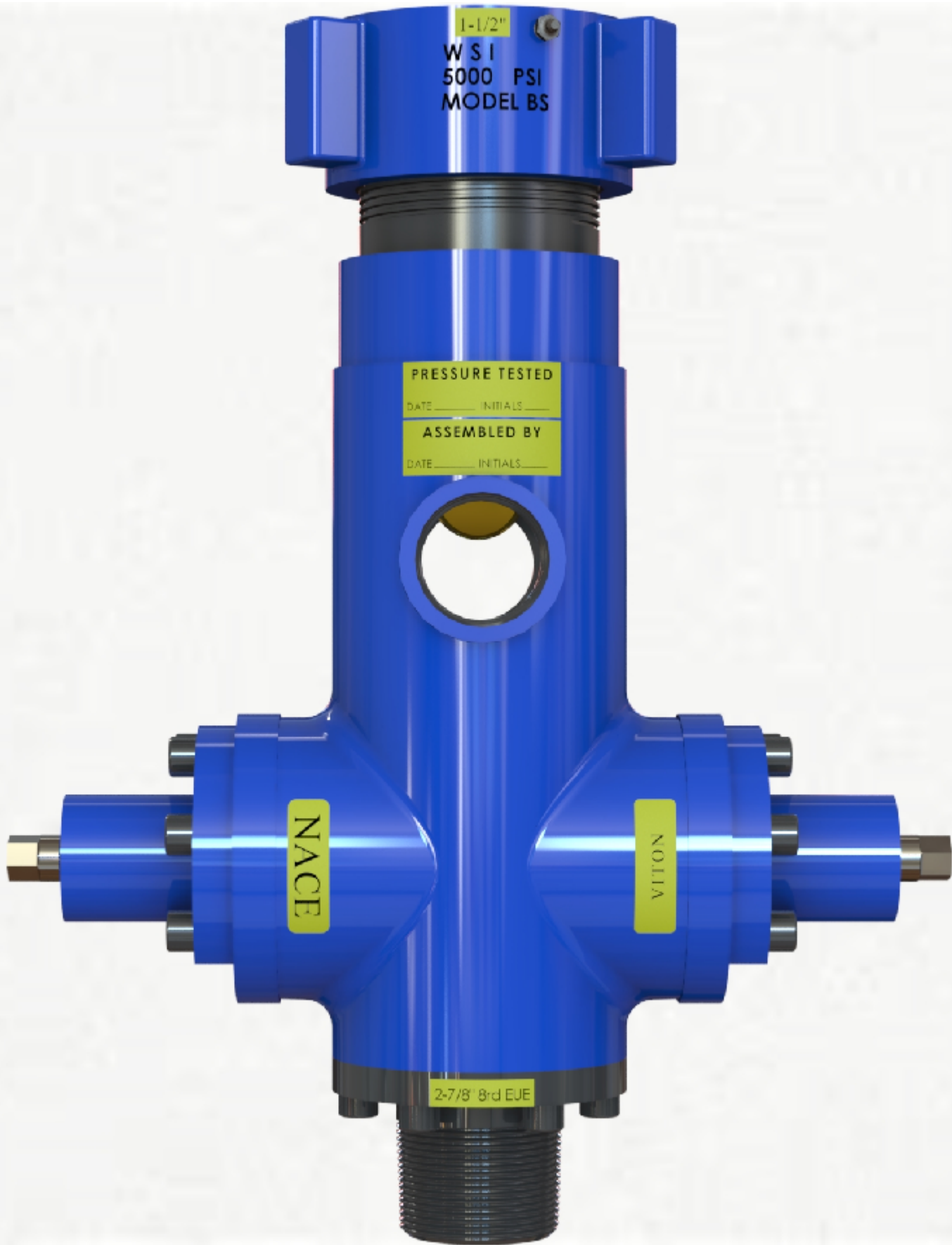
2-7/8" 8rd EUE X 1-1/2" 5,000PSI Model "J-Tee" BOP/SB Complete w/ 2" LPOs, Flapper, HSN Super Dome™ REV C
